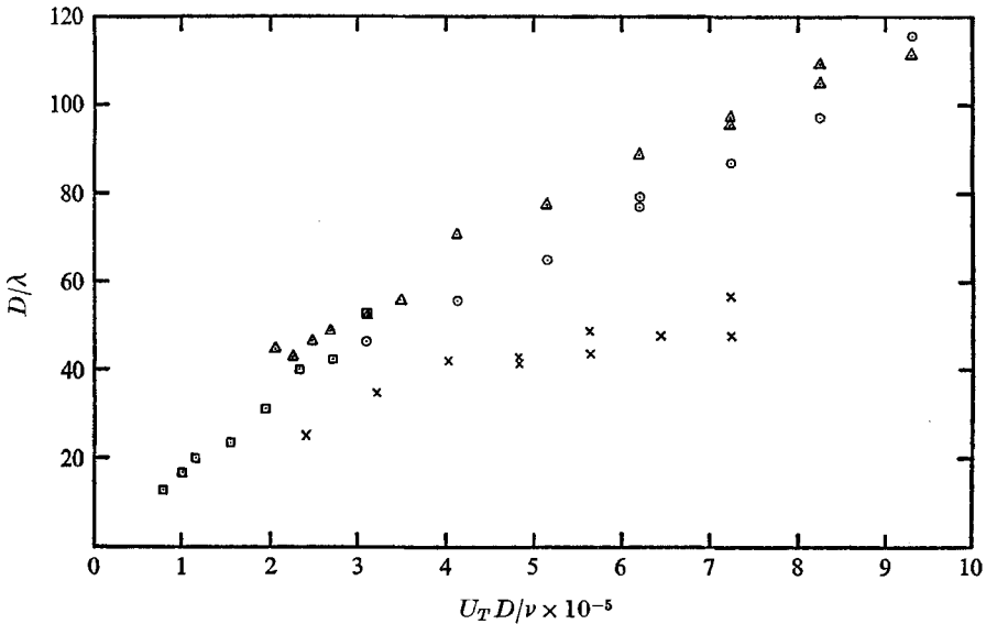
FIGURE 3. Variation of measured wavelengths, \lambda , with tunnel velocity, U_T : ○, 3 in. sphere; △, cutaway sphere; □, 1½ in. sphere; ×, ogive.
