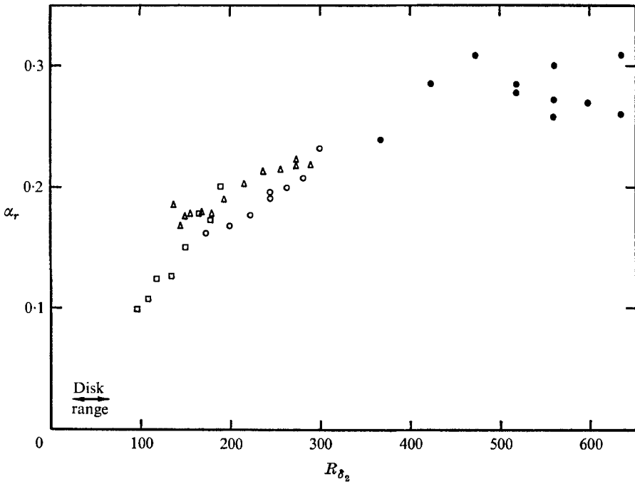
FIGURE 9. The results of figure 3 in dimensionless form; \odot , 3 in. sphere; \triangle , cutaway sphere; \square , 1\frac{1}{8} in. sphere; \bullet , ogive. The range of Reynolds number in which the disk operates is indicated by the arrows.
