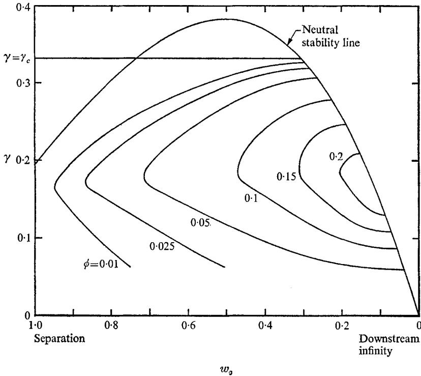
FIGURE 8. Integration of the linear stability characteristics yields \phi = 1/R_{\delta_2} \ln(A/A_s) as a function of \gamma and w_c .
