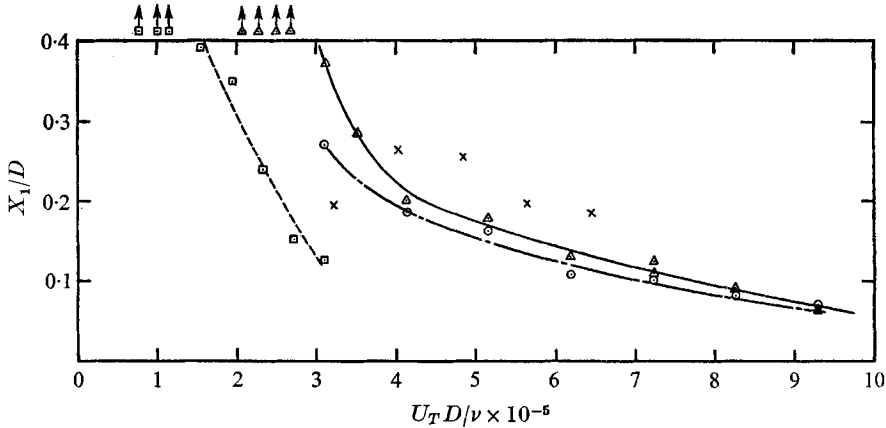
FIGURE 4. Variation of measured distance to wave break up, X_1 , with tunnel velocity, U_T : —○—, 3 in. sphere; —△—, cutaway sphere; --□--, 1½ in. sphere; ×, ogive. Speeds for which virtually no break up occurred are marked with the arrows.
